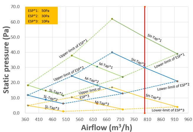
Figure 9.15: MIH45T3HN18
