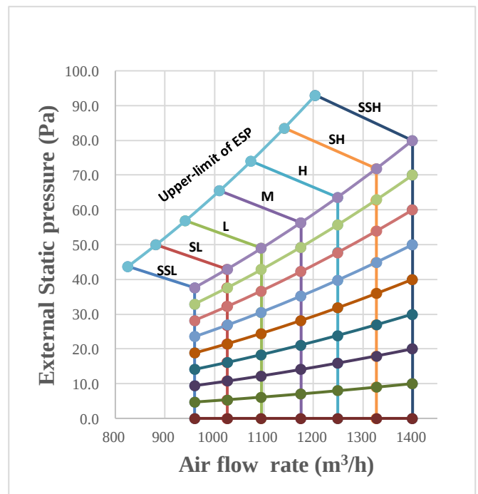
Figure 9.8: MIH80T3HN18
