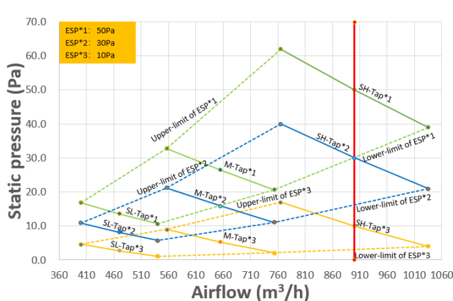
Figure 9.16: MIH56T3HN18
