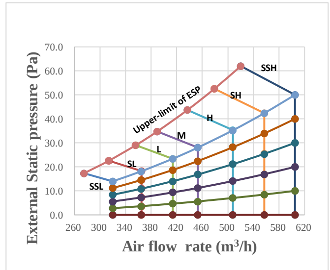
Figure 9.6: MIH56T3HN18
