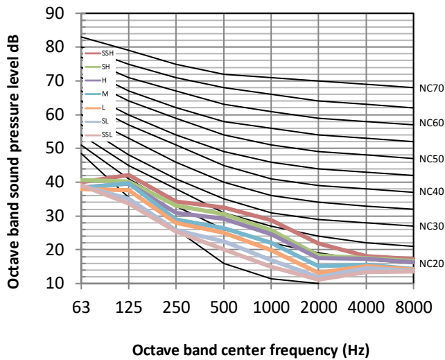
Figure 8.7: MIH45T3HN18 octave band levels
