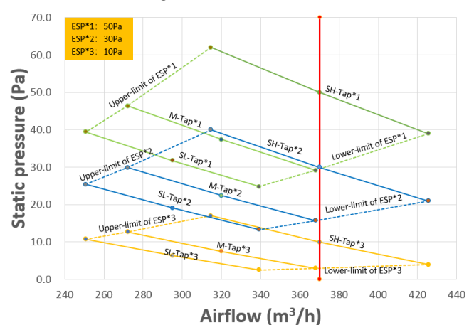
Figure 9.12: MIH22T3HN18
