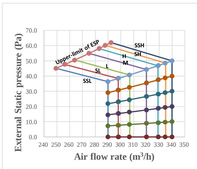
Figure 9.1: MIH15T3HN18
