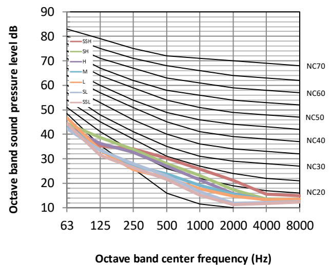
Figure 8.6: MIH36T3HN18 octave band levels
