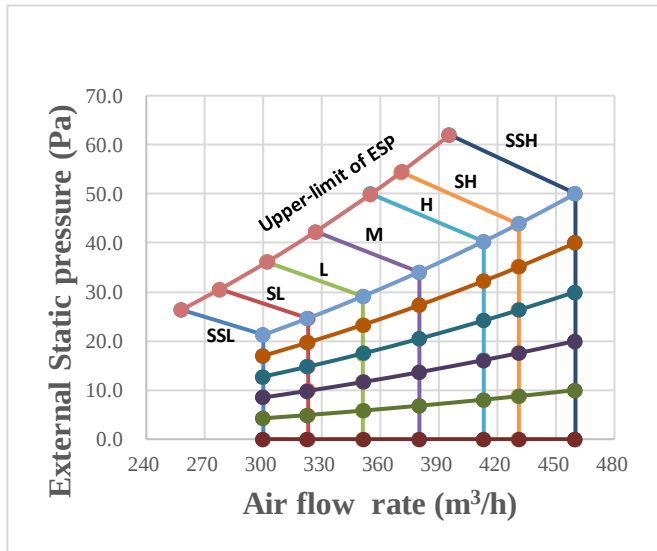
Figure 9.5: MIH45T3HN18
