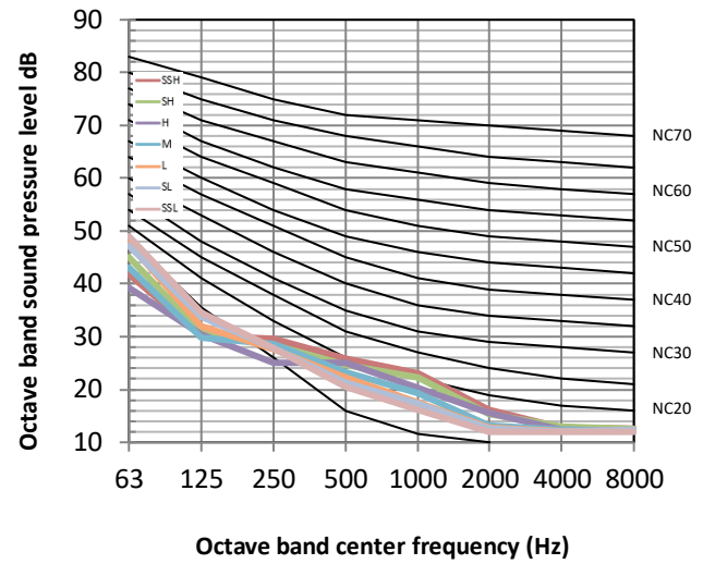
Figure 8.4: MIH22T3HN18 octave band levels
