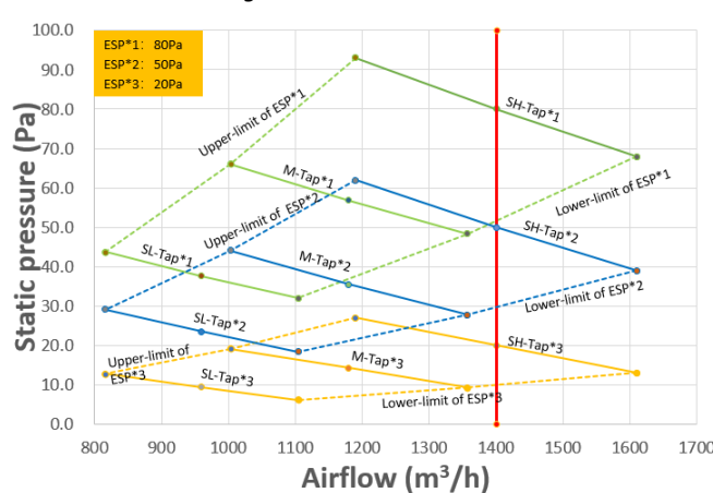
Figure 9.18: MIH80T3HN18
