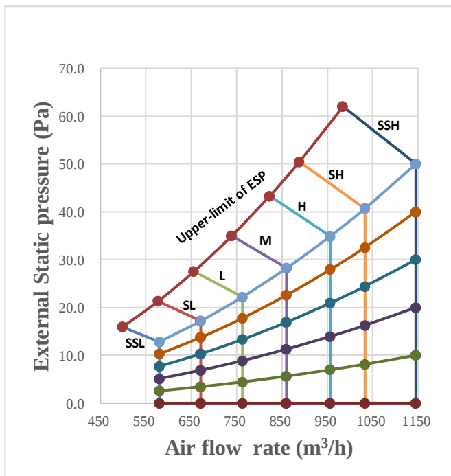
Figure 9.7: MIH71T3HN18
