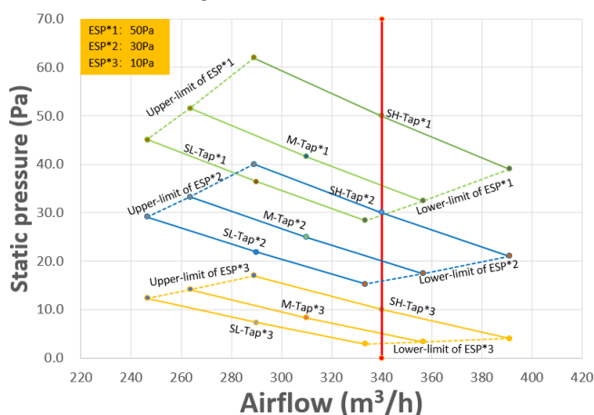
Figure 9.11: MIH15T3HN18
