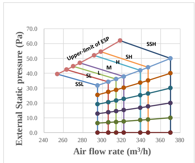
Figure 9.2: MIH22T3HN18
