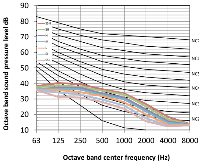
Figure 8.11: MIH90T3HN18 octave band levels
