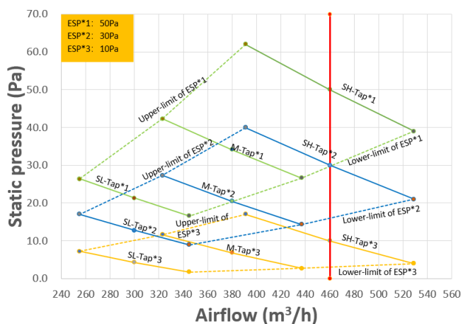
Figure 9.13: MIH28T3HN18
