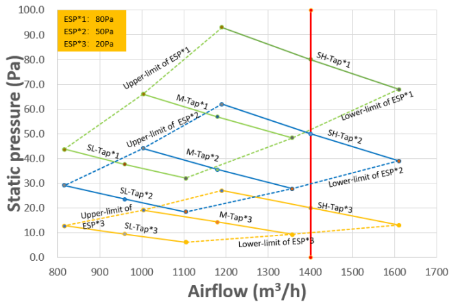
Figure 9.19: MIH90T3HN18
