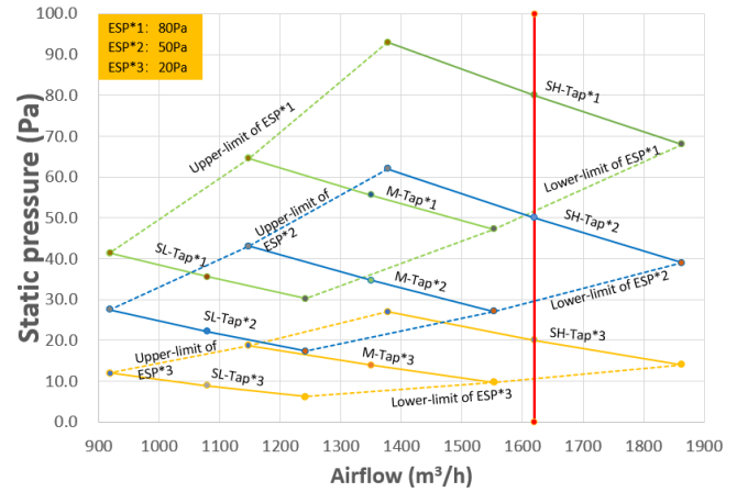
Figure 9.20: MIH112T3HN18
