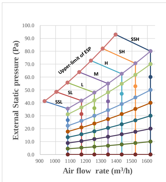
Figure 9.10: MIH112T3HN18
