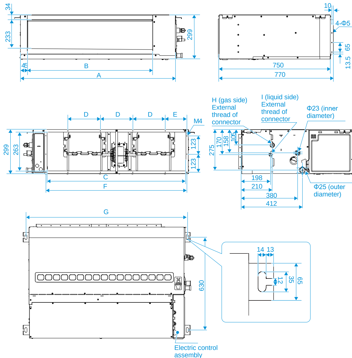
Figure 2.1: MIH56(71,80,90,112,125,140,160)T1HN18 dimensions (unit: mm)
