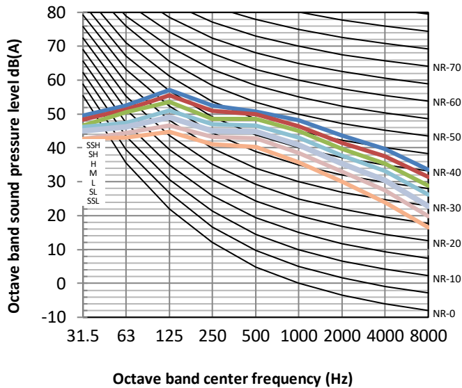
Figure 8.8: MIH200T1HN18 octave band levels
