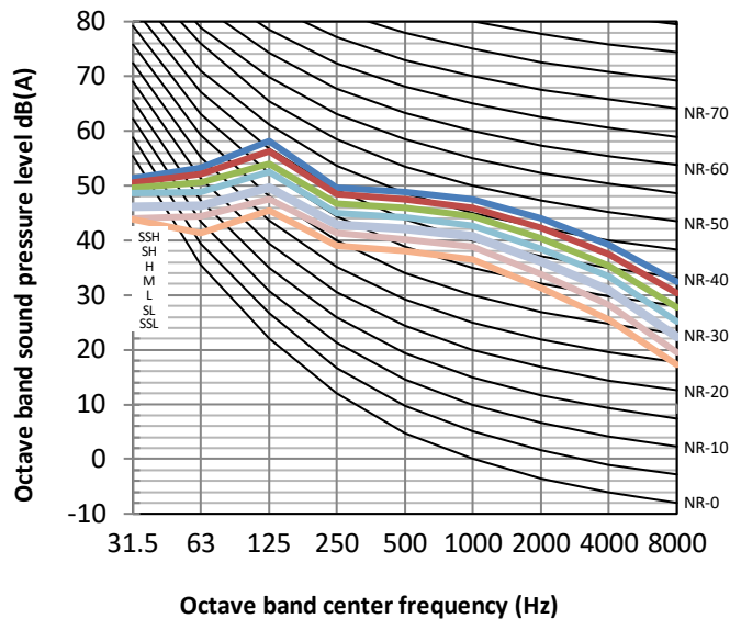
Figure 8.12: MIH335T1HN18 octave band levels
