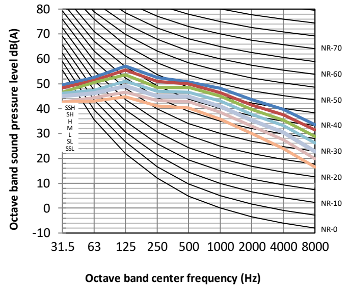
Figure 8.9: MIH224T1HN18 octave band levels
