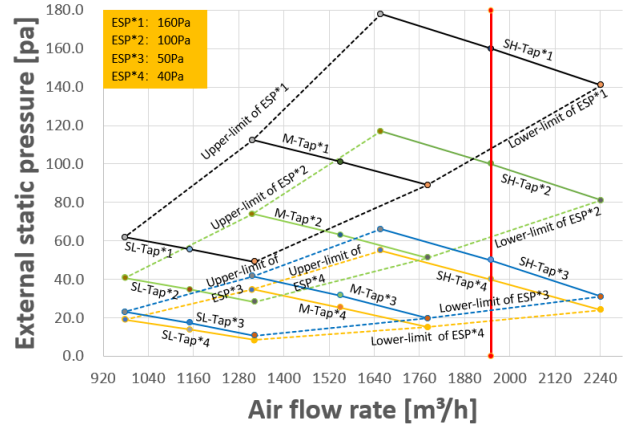
Figure 9.22: MIH112T2HN18
