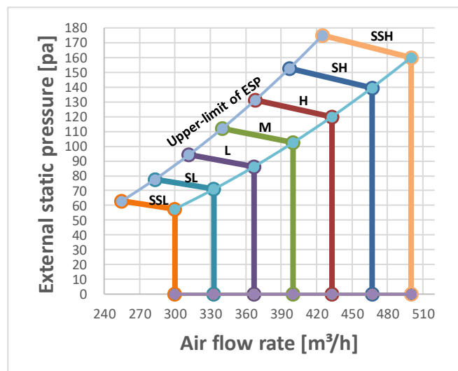
Figure 9.2: MIH22T2HN18
