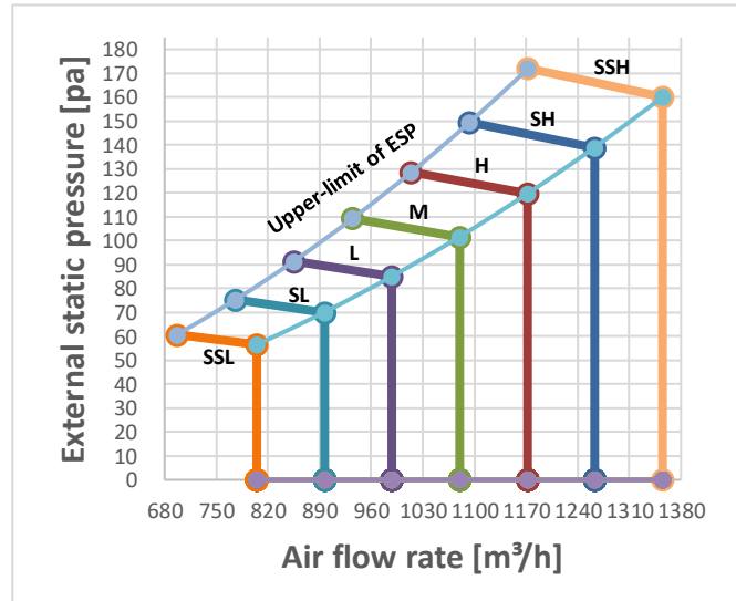
Figure 9.8: MIH80T2HN18
