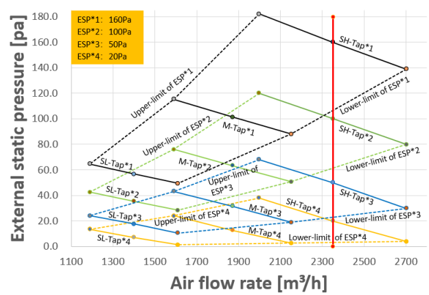
Figure 9.24: MIH160T2HN18
