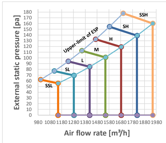
Figure 9.10: MIH112T2HN18
