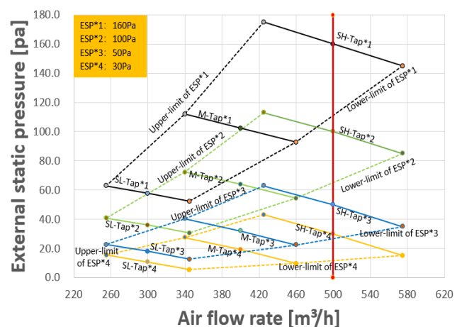
Figure 9.14: MIH22T2HN18
