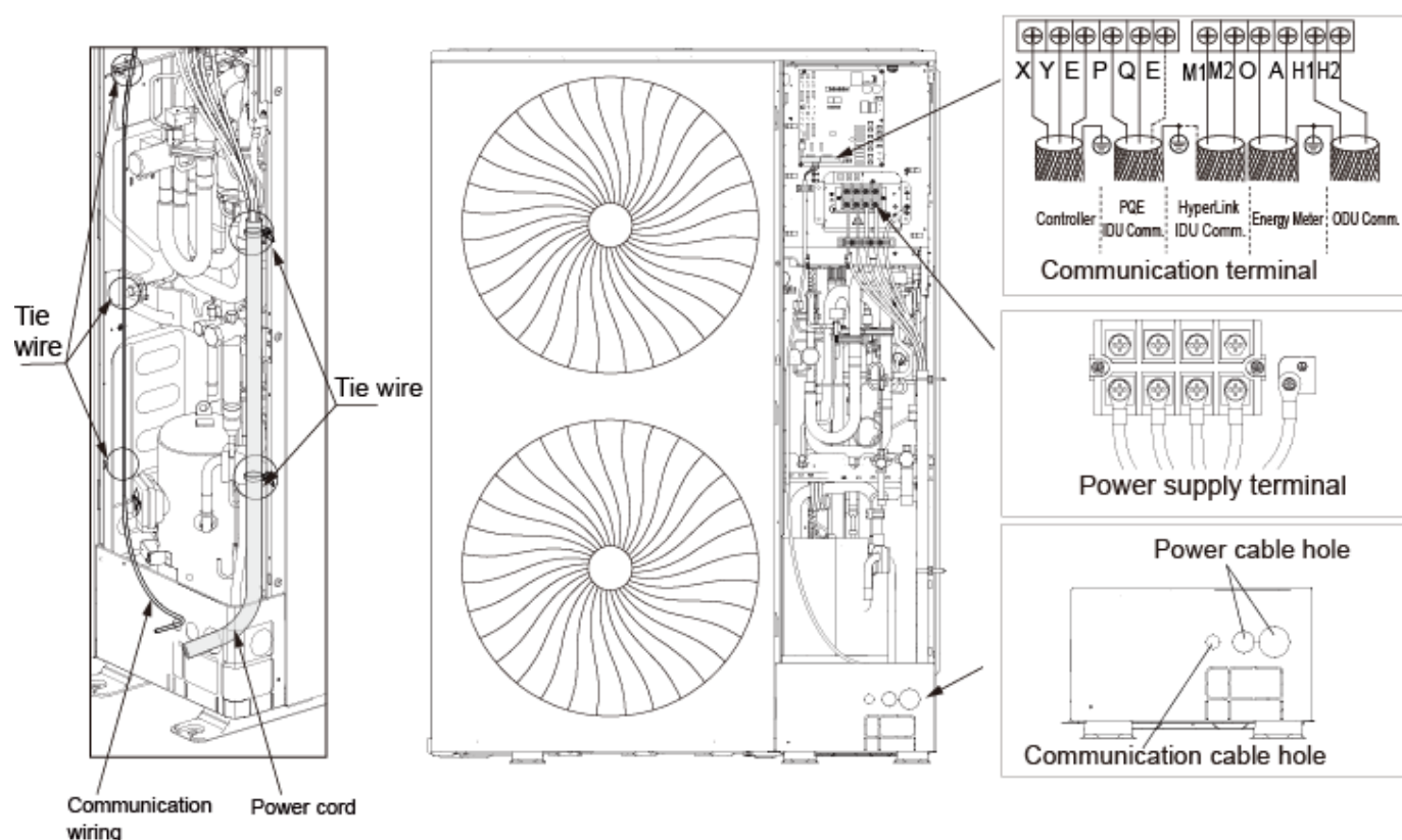
Figure 3-9.1: Wiring layout
