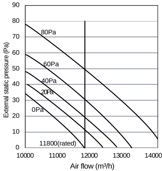
Figure 3-3.2: 8HP units fan performance
