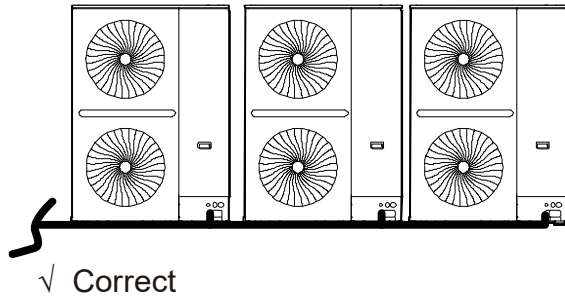
Figure 3-5.13: Piping connections between outdoor units
