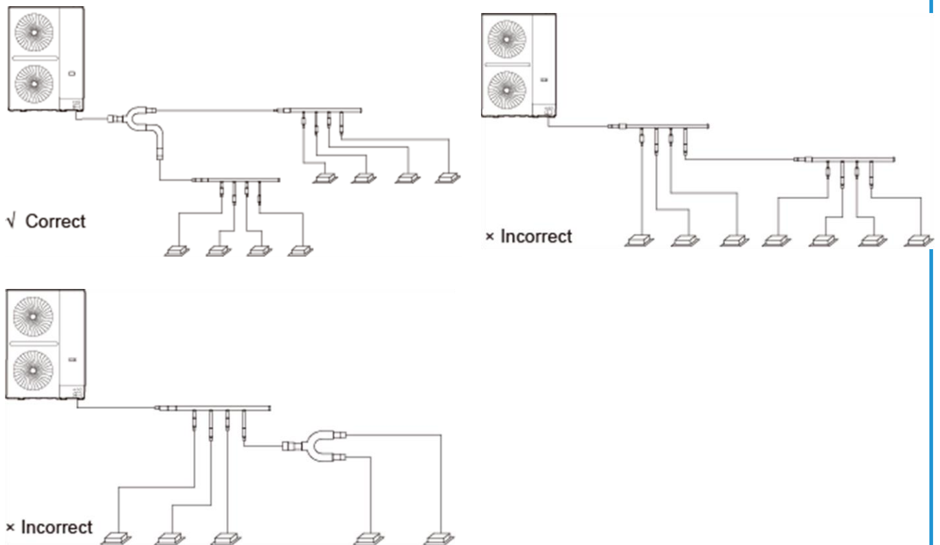
Figure 3-5.11: Installation of outdoor branch joints
