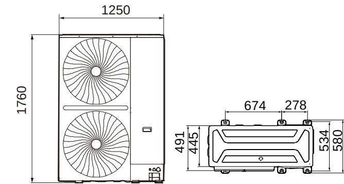
Figure 2-2.2: 16/18/20/22HP dimensions (unit: mm)
