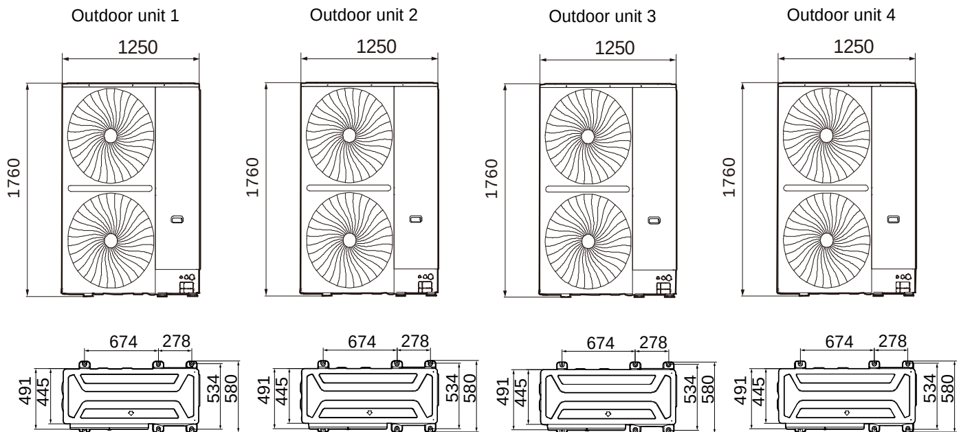
Figure 2-2.12: 72/74/76/78/80/82/84/86/88HP dimensions (unit: mm)
