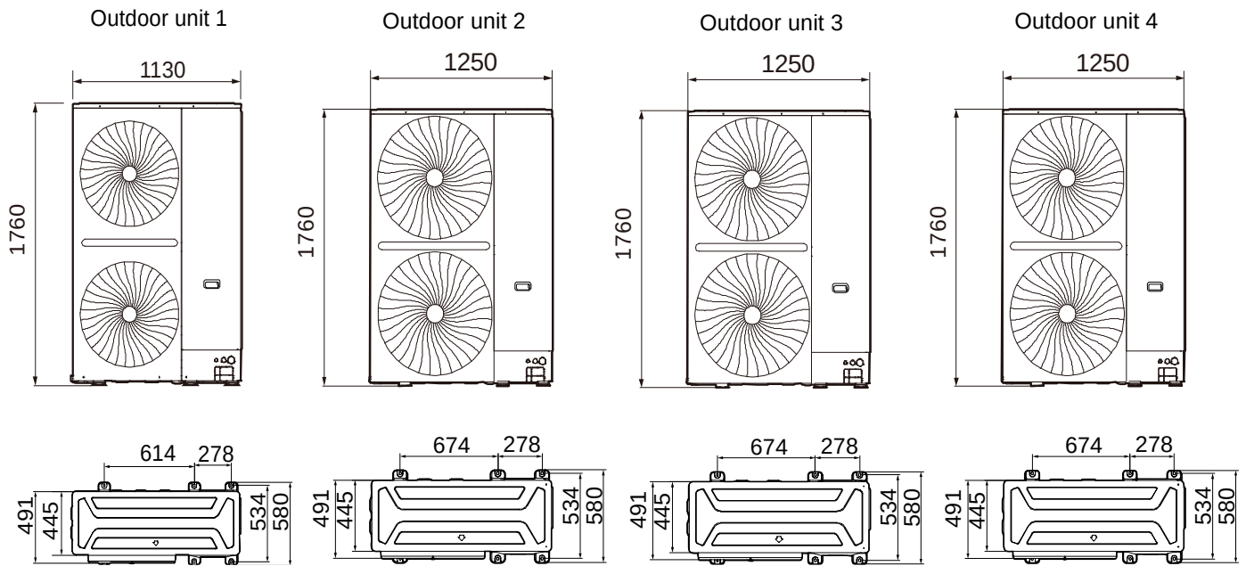
Figure 2-2.11: 68/70HP dimensions (unit: mm)
