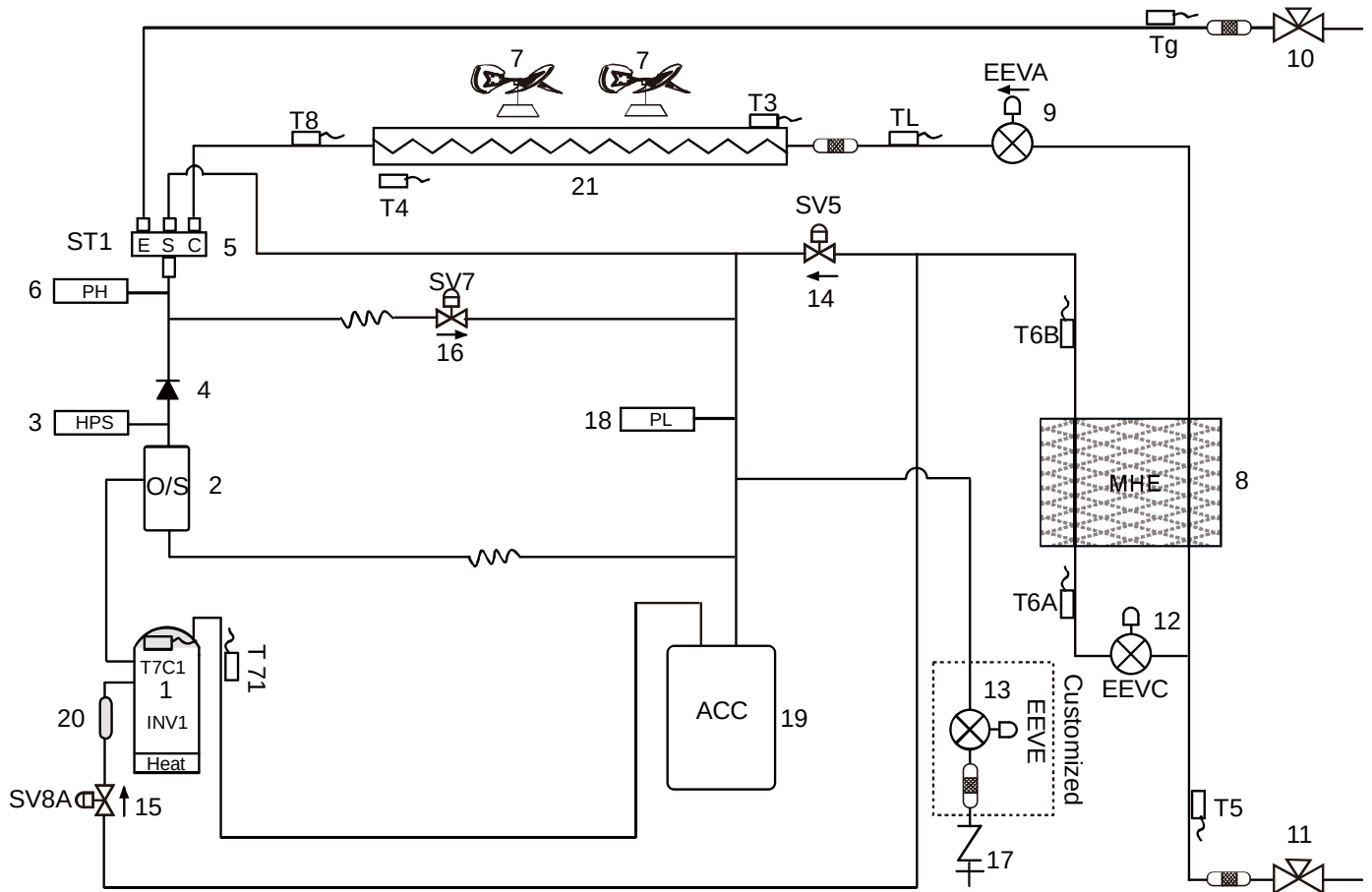
Figure 2-4.1: 8-14HP piping diagram
