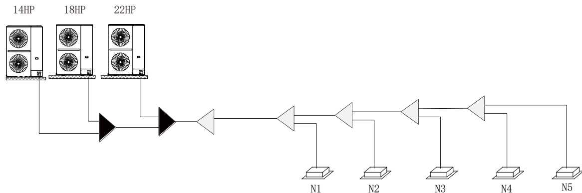
Figure 3-2.1: Positioning of master and slave units
