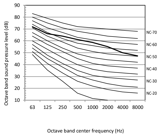
Figure 2-10.9: 22HP octave band level
