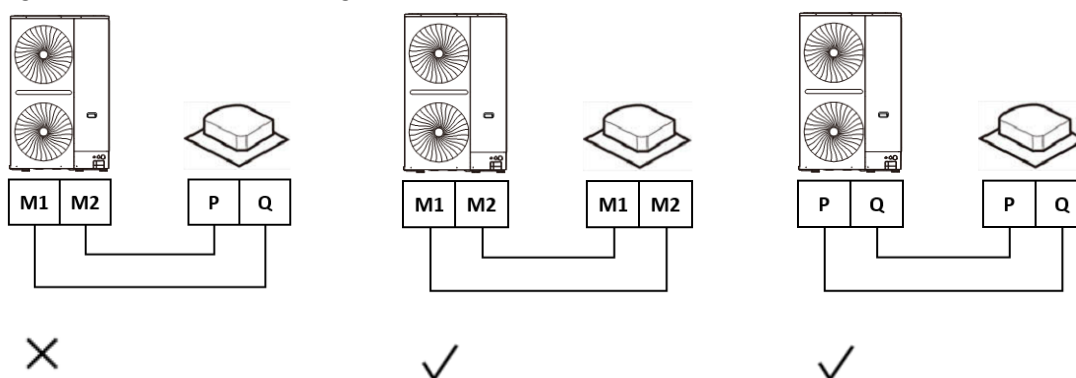
Figure 3-9.5: Communication wiring
