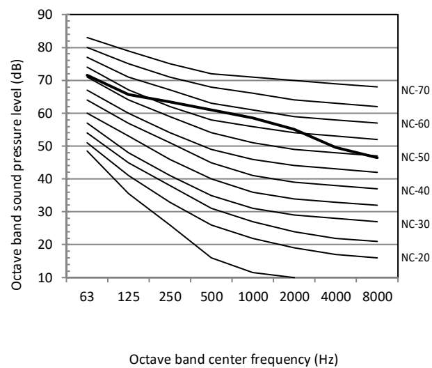
Figure 2-10.8: 20HP octave band level
