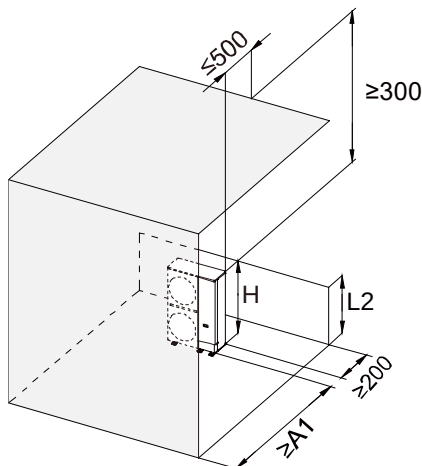
Figure 2-3.11: One outdoor unit installation (unit: mm)
