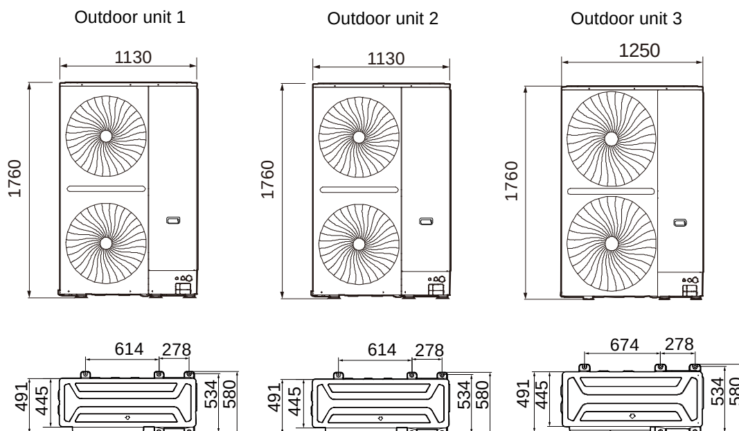
Figure 2-2.8: 46HP dimensions (unit: mm)
