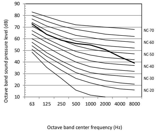
Figure 2-10.3: 10HP octave band level
